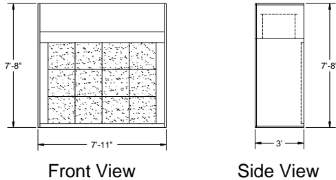
Exhaust Box
